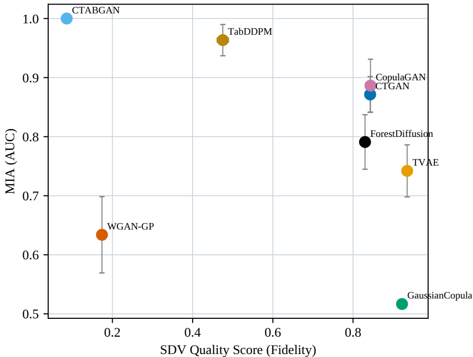
Forest Cover: SDV Quality Score (Fidelity) vs MIA (AUC)
